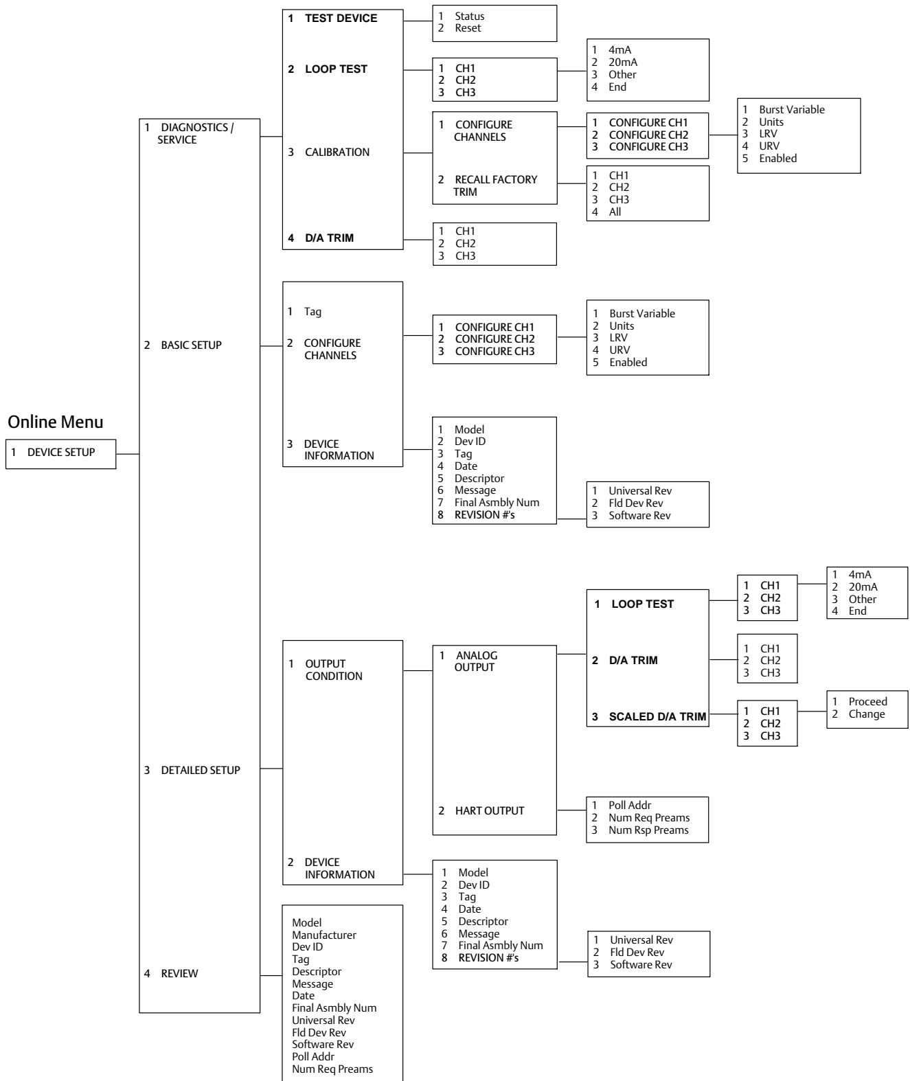
Figure 2. Menu Tree for the Tri-Loop Signal Converter
